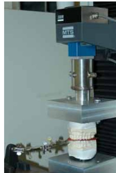
Fig. (2). MTS testing machine - closed with casts intercusped and articulating paper horseshoe interposed.
